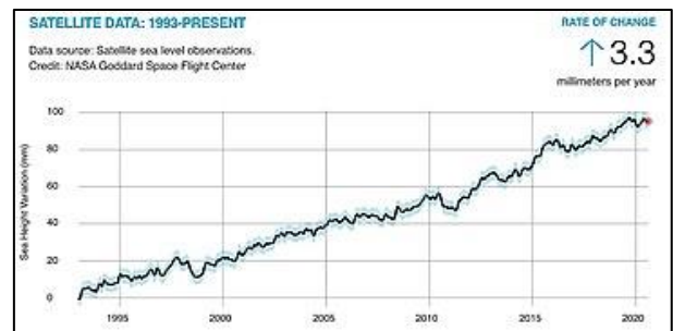
Sea level change in mm per year from 1993 to 2020 based on satellite data. (NASA – in the public domain).
