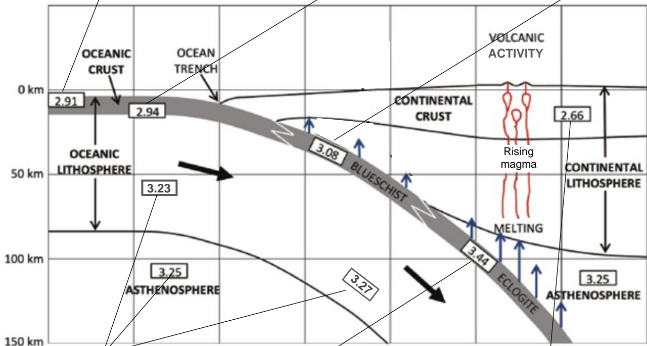
Basalt, density around 2.91\text{gcm}^{-3}
