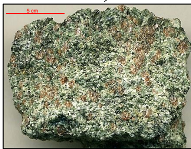
Eclogite, density around 3.44\text{gcm}^{-3}
